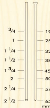
166A. FINISH NAILER PR-1664T
